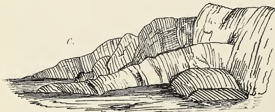
a. Fragments imbedded in Granite b. Granite with twisted veins. c. Stratified rocks protruded through Granite
